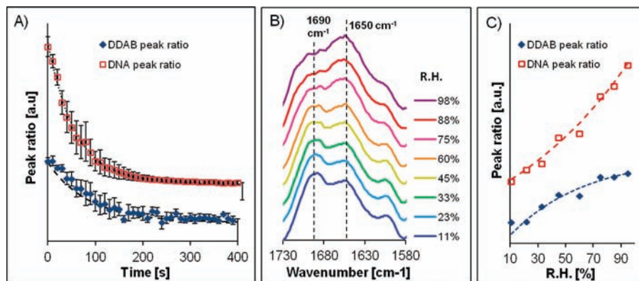
Figure 1. (A) Summary of FT-IR spectra of the DNA base pair region taken every 10 s as a water-immersed film dried for 400 s. Decrease in the peak ratios of 1690 to 1650 \text{cm}^{-1} of the DNA base pair and DDAB tail regions averaged over four sequential measurements with error bars showing the standard deviation for each point. The DDAB values are amplified by a factor of 60 compared to the DNA values for comparison purposes. The peak ratio decreases (and therefore the structural switching of DNA and DDAB) occur virtually simultaneously, as indicated in the k values of the exponential curve fit. The curve fit for the DNA peak ratio is y = 1.577 + 2.563 \cdot e^{(-0.017 \cdot \text{time})} and the curve fit for the DDAB peak ratio is y = 0.846 + 1.098 \cdot e^{(-0.011 \cdot \text{time})} . (C) FT-IR spectra of the DNA base pair region of a cast film at different relative humidity (R.H.) levels showing the gradual transition from ssDNA (11% R.H.) to dsDNA (95% R.H.). Dotted lines indicate the peak positions at 1650 and 1690 \text{cm}^{-1} . (D) Peak ratio intensities of the DNA base pair and DDAB tail regions increase with increasing humidity levels, again showing the nearly simultaneous structural transition of DNA and DDAB.
