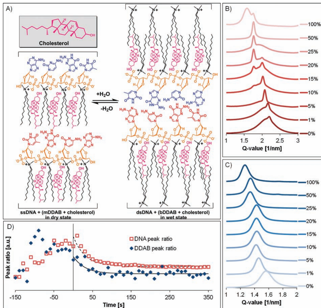
Figure 5. Cholesterol-blended DNA-DDAB films. (A) Expected structural change of the cholesterol-doped films between the dry and wet states. Cholesterol is shown in pink, inserted between the DDAB aliphatic tails though both DNA and DDAB are able to switch. (B) SAXS spectra of dry films with varying amounts of cholesterol. (C) SAXS spectra of the same films in the wet state. Both sets of data indicate that the lamellar spacing of the films increases with increasing amounts of cholesterol. Peak ratios in the DNA base-pair and DDAB tail regions of dry cholesterol films (see Figure S11 in the Supporting Information) indicate that DDAB remains largely in a bilayer while DNA becomes more double-stranded with increasing amounts of cholesterol, presumably due to the increased retention of water by cholesterol in the film. (D) Variations in the DNA and DDAB peak ratios in their respective regions over time in a wetted 20% cholesterol film as it dried. K values for the process are approximately triple that of normal DNA-DDAB films. The gray line indicates time of addition of water.
