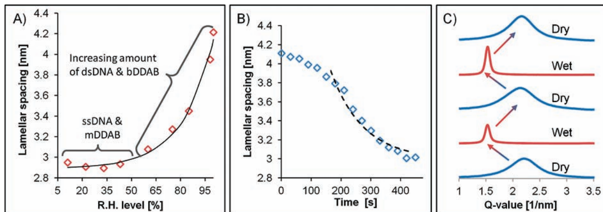
Figure 2. Small angle X-ray (SAXS) scattering of the DNA-DDAB films at various humidity levels. An increase in humidity leads to a structural swelling of the film with a correspondingly increasing lamellar spacing (A). The black dotted line indicates the shift of the main scattering peak with increasing humidity. The transition begins to occur more dramatically at a threshold value of approximately 60% R.H. which agrees with FT-IR measurements. The exponential curve fit is y = 0.01 \cdot e^{0.05x} + 2.90 . The timing of this transition was monitored by synchrotron SAXS experiments using a water-immersed cast film. The black line indicates the position of the main scattering peak at various humidity levels (B). The slope of the decrease in lamellar spacing as the film dries is nearly identical to the slope of the decrease in peak ratios measured by FT-IR, indicating that the two techniques are sufficiently comparable and that the timing of the film's switching is unchanged regardless of drying conditions and film thickness. The structural transition caused by hydration and dehydration is fully reversible (C) which could be seen in the identical peak width and q -value for all wet and dry films, respectively.
