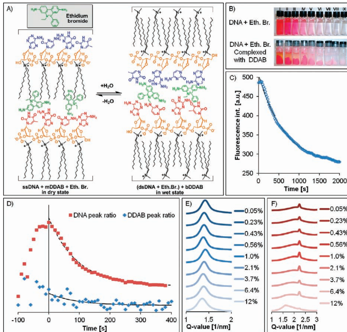
Figure 6. Structural analysis of ethidium bromide-labeled films. (A) Expected structural change of the DNA-DDAB film with added ethidium bromide between the dry and wet states. Ethidium bromide is shown in green, intercalating between the DNA base-pairs in the wet state, while it associates both with the exposed hydrophobic DNA bases and DDAB tails in the dry state. (B) Photographs of aqueous solutions or suspensions of (top) DNA with varying amounts of ethidium bromide and (bottom) DNA-DDAB complexes labeled with ethidium bromide. The supernatant used in the UV-vis studies to measure the amount of ethidium bromide intercalation is the liquid taken from the bottom row of suspensions (see Supporting Information, Figure S13). The numbers I-IX refer to varying percentages 0.05–12% ethidium bromide, respectively. (C) Decay in fluorescence over time of a wetted 6.4% ethidium bromide-labeled film as it dried, agreeing with earlier data that suggests DNA is double-stranded in the wet film and becomes single-stranded in the dry film, and thus can no longer intercalate ethidium bromide which can then no longer fluoresce. Curve fitting indicates that the decay is exponential. (D) Variations in the peak ratio of a 6.4% ethidium bromide wetted film as it dries over time fitted with an exponential curve equation. K values for both DNA and DDAB ratio decay are nearly identical to that of the normal DNA-DDAB films (see Figure 1). (E) SAXS spectra of wet films labeled with varying amounts of ethidium bromide. (F) SAXS spectra of the same films in the dry state.
