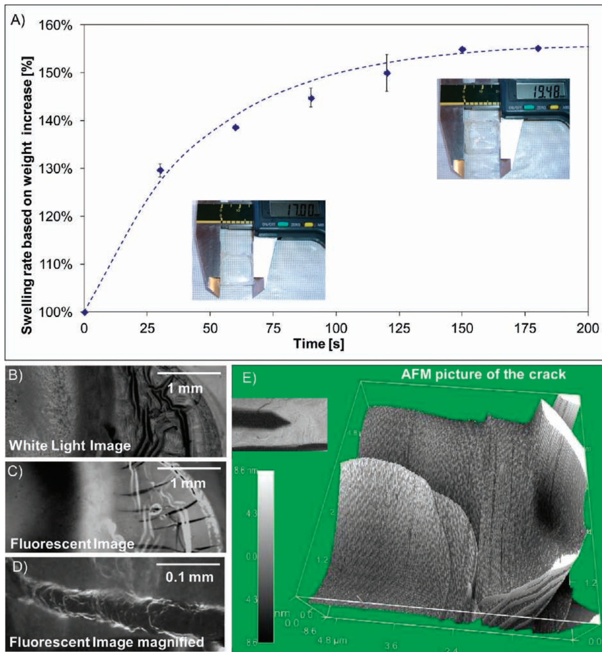
Figure 7. Macroscopic swelling and degradation experiments of a cast film. The molecular transition between dry and wet films can also be observed in a thick film when the dry film is immersed in water, based on weight and size increase. (A) Increase of 155% in volume corresponds to the transition from the structure in dry state to the structure in wet state, which is the same percent increase in the lamellar spacing from the dry to wet film (2.8 to 4.4 nm), indicating a direct correlation between the macroscopic and nanoscopic film structure. The rate was determined with an exponential fit to y = 1.562 - 0.5528 e^{(-0.2147 \cdot \text{time})} which is comparable to the drying rate. (B–D) Fluorescent and white light images of an ethidium bromide-labeled film on top of which was added PBS buffer, causing the film to degrade. (B) White light microscope image of the area in which the buffer was added. (C) Fluorescent microscope image of the same region, showing the DNA aggregation (bright areas) separated from the DDAB (dark areas). (D) Close-up of the cracks at the edge of the PBS region, indicating step formation. (E) Analysis of the cracks in the film by AFM indicates that the film degrades layer by layer, as the steps are \sim 2.8 nm in height.
