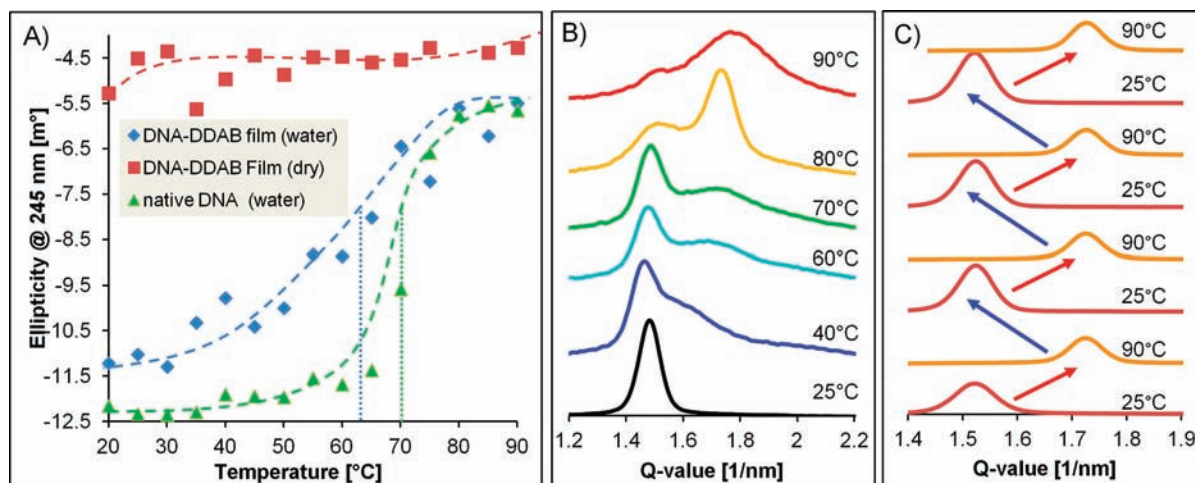
Figure 3. Temperature response of the DNA-DDAB films. By comparing the peak value at 245 nm in the CD-spectra of native DNA and a wet and dry film during the same heating process and using a Boltzmann curve fitting (A), the melting temperature of DNA in the wet film is \sim 63.1 °C, compared to \sim 71.2 °C for native DNA, a decrease presumably due to complexation of DNA by DDAB which reduces backbone repulsion between the two strands which would lower the melting point. The T values for each curve indicate the broadness (i.e., the homogeneity of helical DNA), as measured in degrees Celsius, of the DNA melting point. No reasonable melting temperature could be obtained for the DNA in the dry film, indicating that it is single-stranded and cannot melt. Similar behavior was noted in the SAXS spectra of wet (B) and dry DNA films (Supporting Information Figure S11). As the temperature increases the q -value of the main scattering peak of the wet DNA-DDAB film increases and the lamellar spacing correspondingly decreases from 4.4 to 3.6 nm, suggesting that the heated wet film consists of bDDAB (2.4 nm) + ssDNA (1.1 nm). The CD results in combination with SAXS (B) experiments of the wet film indicate that the DDAB remains in bilayer formation while the DNA becomes single stranded. The heat treatment, even after several cycles, does not change the structure of the wet film, indicating that it is thermostable (C).
